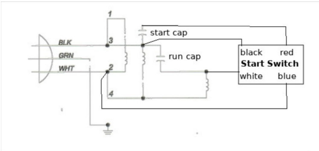
New wiring diagram
